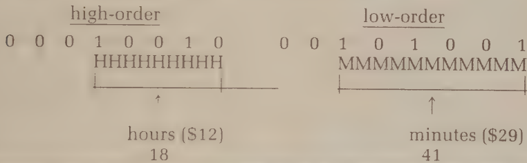
Figure 8-1. The formats of the DATE and TIME bytes.
