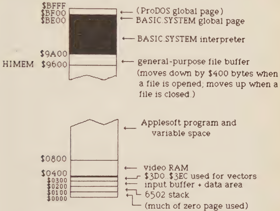
Figure 5-1. BASIC.SYSTEM memory map
