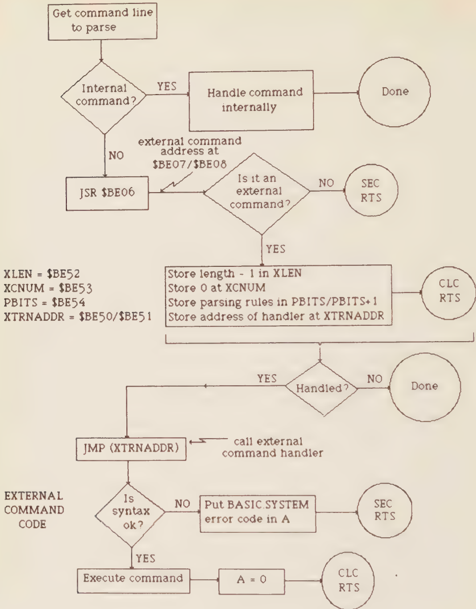
Figure 5-2. A flowchart showing the execution of an external command
