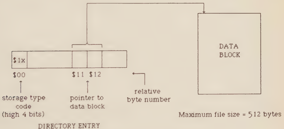
Figure 2-9. The structure of a seedling file
