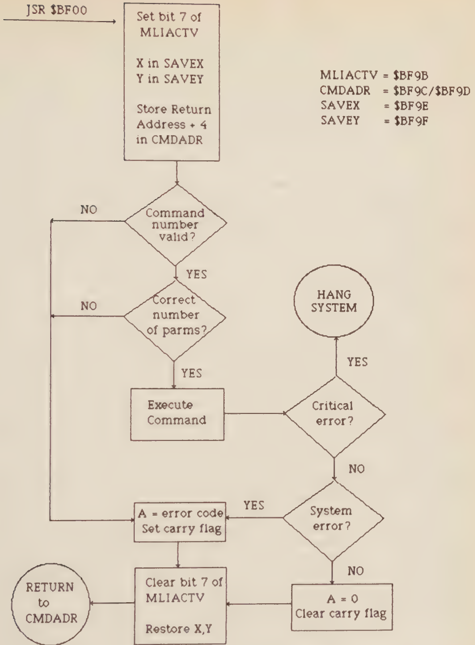
Figure 4-1. A flowchart of MLI operations
