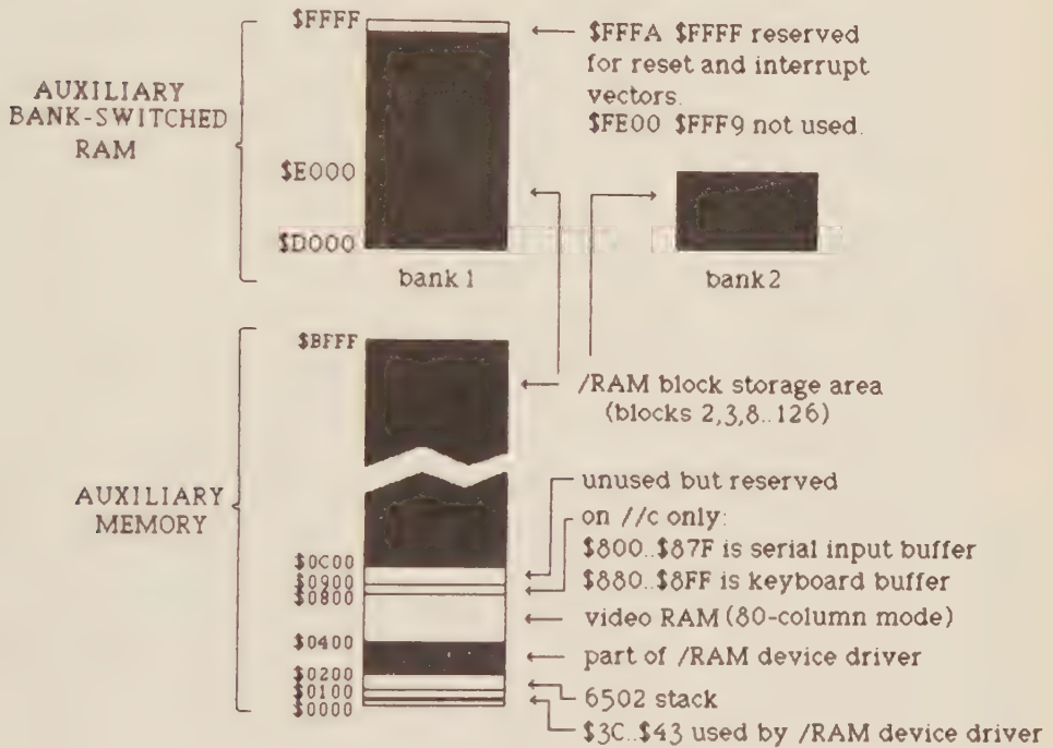
Figure 7-2. A map of auxiliary memory usage on the //e and //c
