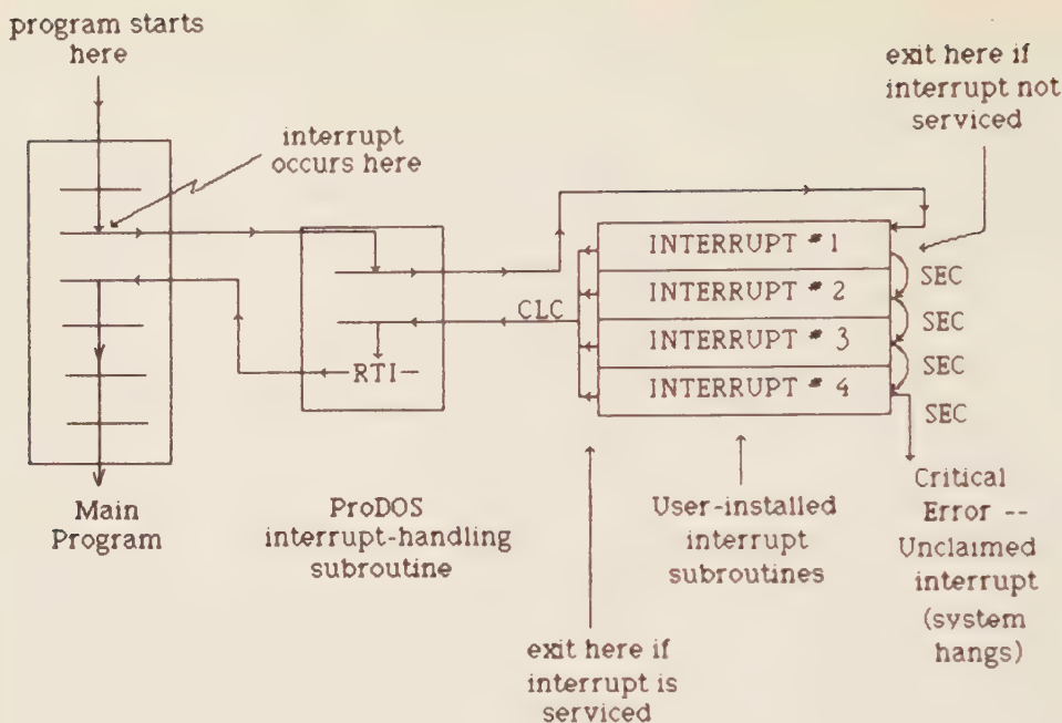
Figure 6-1. How ProDOS handles interrupts
