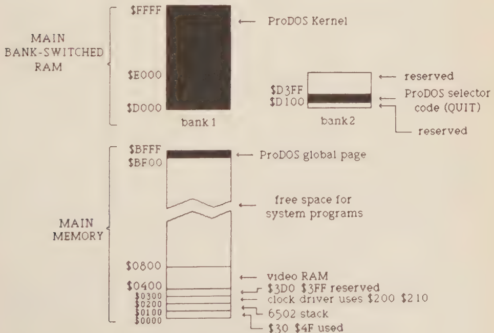
Figure 3-1. ProDOS Memory Map.
