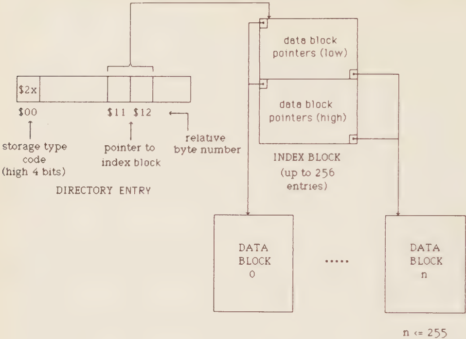
Figure 2-10. The structure of a sapling file
