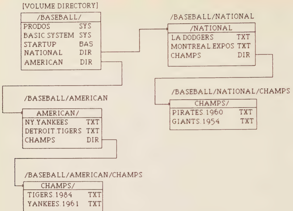
Figure 2-1. Diagram of the BASEBALL directory
